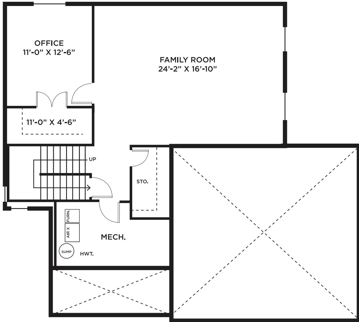
BASEMENT
