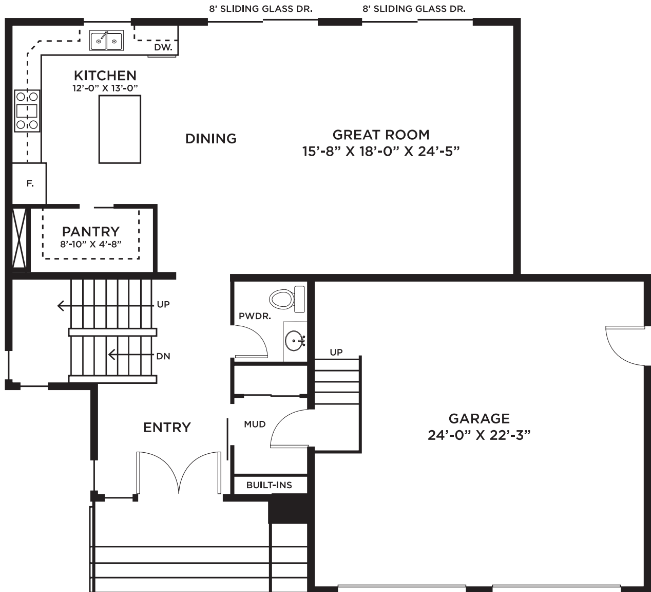
MAIN FLOOR
